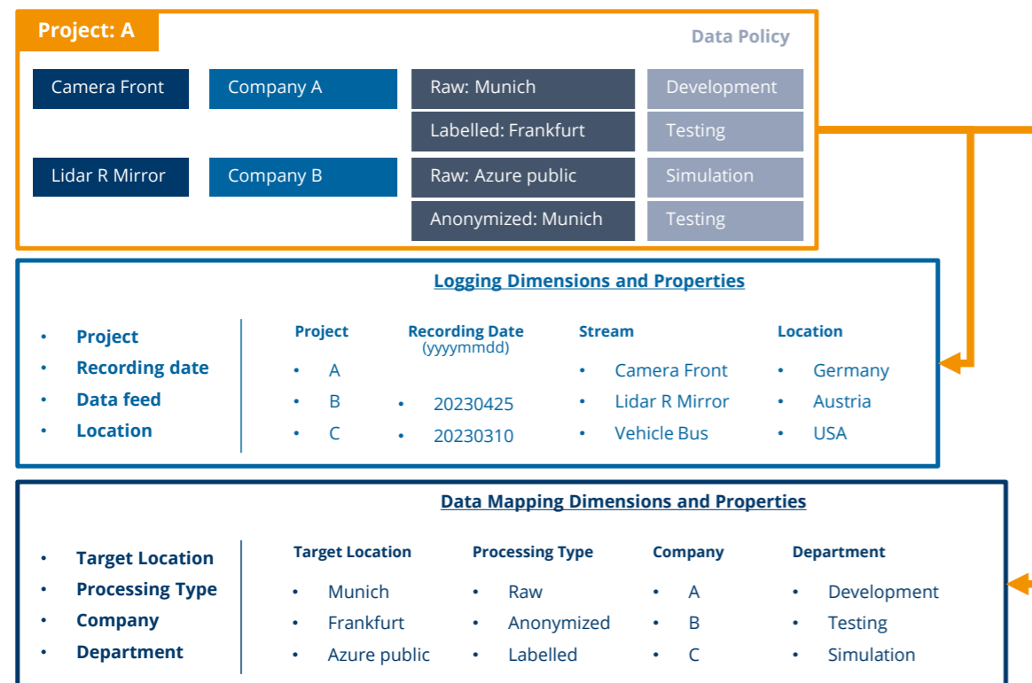
Fig.3: User-defined policies and GADS: The storage, transfer and management of access rights for globally uploaded data is the whole time legally compliant and meets the highest requirements in the automotive industry. With case-optimized access to global data, it is also easy to perform data integrity checks and obtain reliable results for autonomous driving simulation.
